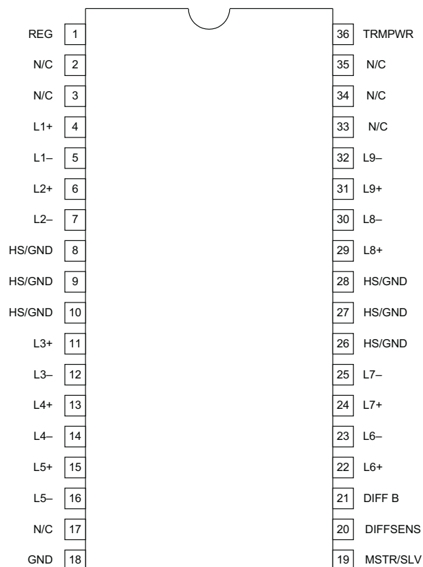
SSOP-36 (Top View) MWP Package
